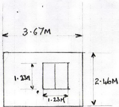
REAR ELEVATION
